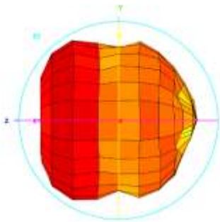
Total_3D_Left View_2.45GHz
